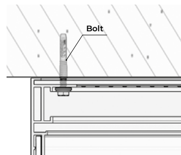
Straight Mounting to Base Ceiling or a Wall
