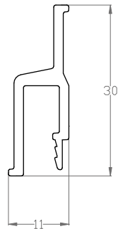
AL 04 basic wall profile used with decoration strip
