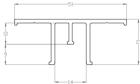
AL 07 A separator anodised profile
