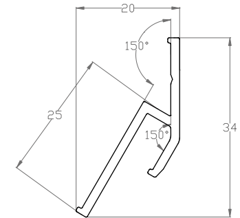
AL 11 constructive profile
