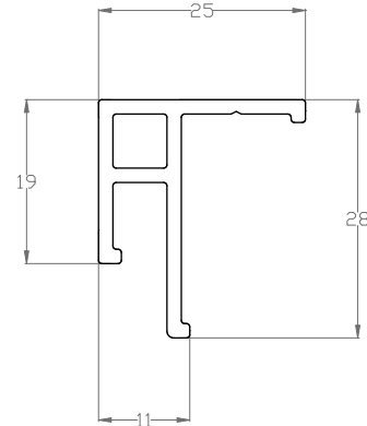
AL 01 S basic universal profile used without decoration strip
