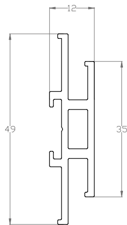
AL 19 Luca modular profile
