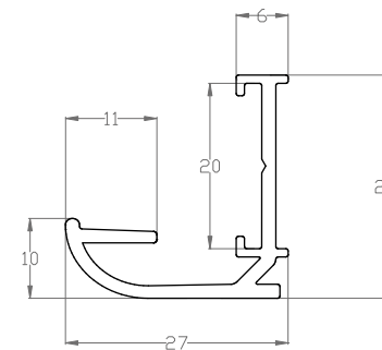
AL 13 W white wall profile
