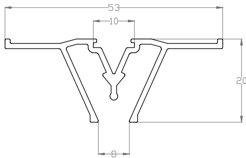
AL 03 separator profile
