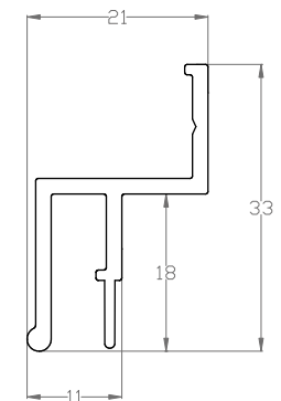
AL 14 modular and lighting profile
