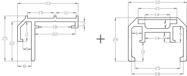
AL 36 A modular and lighting anodised profile
