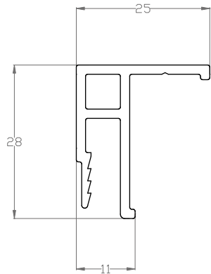
AL 01 basic universal profile used with decoration strip
