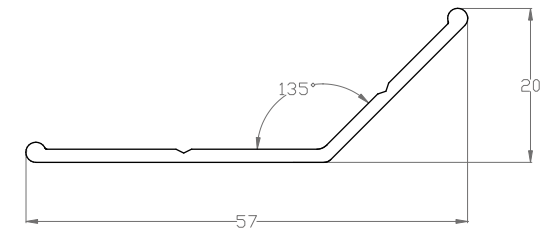
AL 06 A constructive anodised profile
