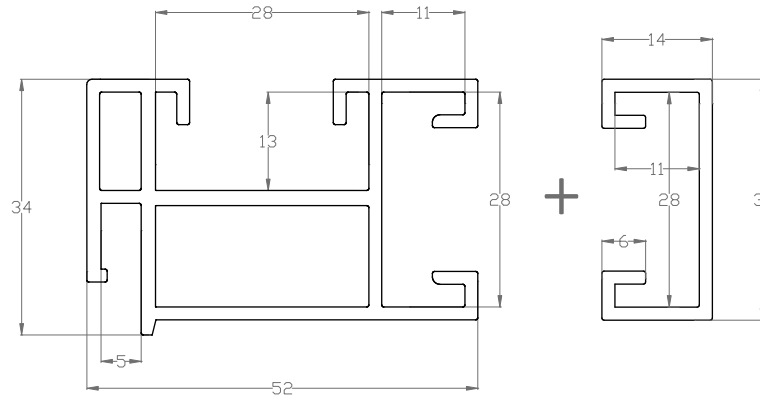
AL 16 W white modular profile
