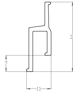
AL 05 basic wall profile used without decoration strip
