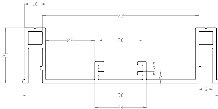
AL 12 W white separator profile
