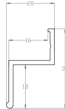
AL 10 A constructive anodised profile
